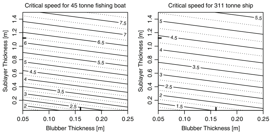
FIGURE 5 Dependence of the critical vessel speed, in knots, on the thickness of blubber and sublayer, for a 45-tonne fishing boat with impact area 1.32 \text{ m}^2 (left) and a 311-tonne ship with impact area 0.88 \text{ m}^2 (right). The contours show the collision speed that yields a compression stress that corresponds with P(\text{lethal}) = .5 . The tick marks inside the axes show the default layer thickness values of the model, which are intended to represent a mid-body ship strike of a right whale. The velocities at the intersections of these tick marks match those at stress \tau_{50} in Figure 4.
